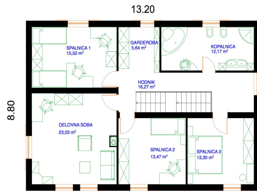
MANSARDA
