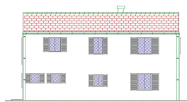
FASADA SEVER
